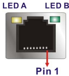
Figure 6-19: LAN Connector
